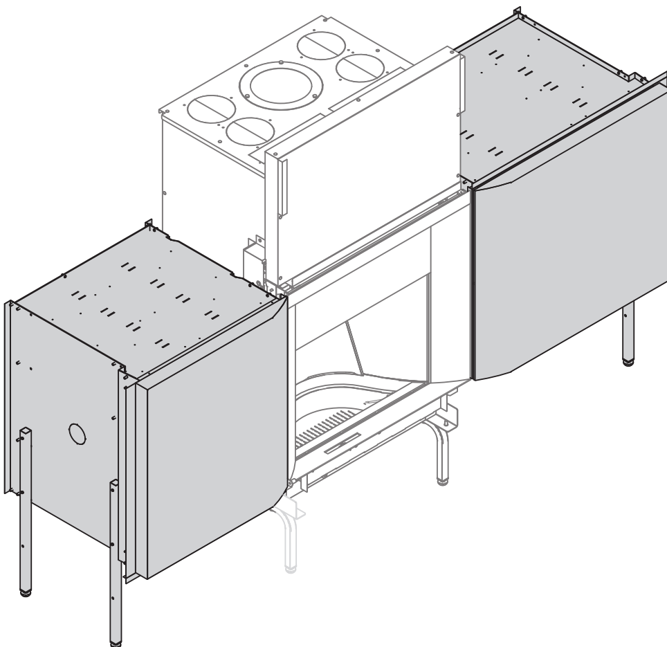
ASYMMETRISCH LINKS
